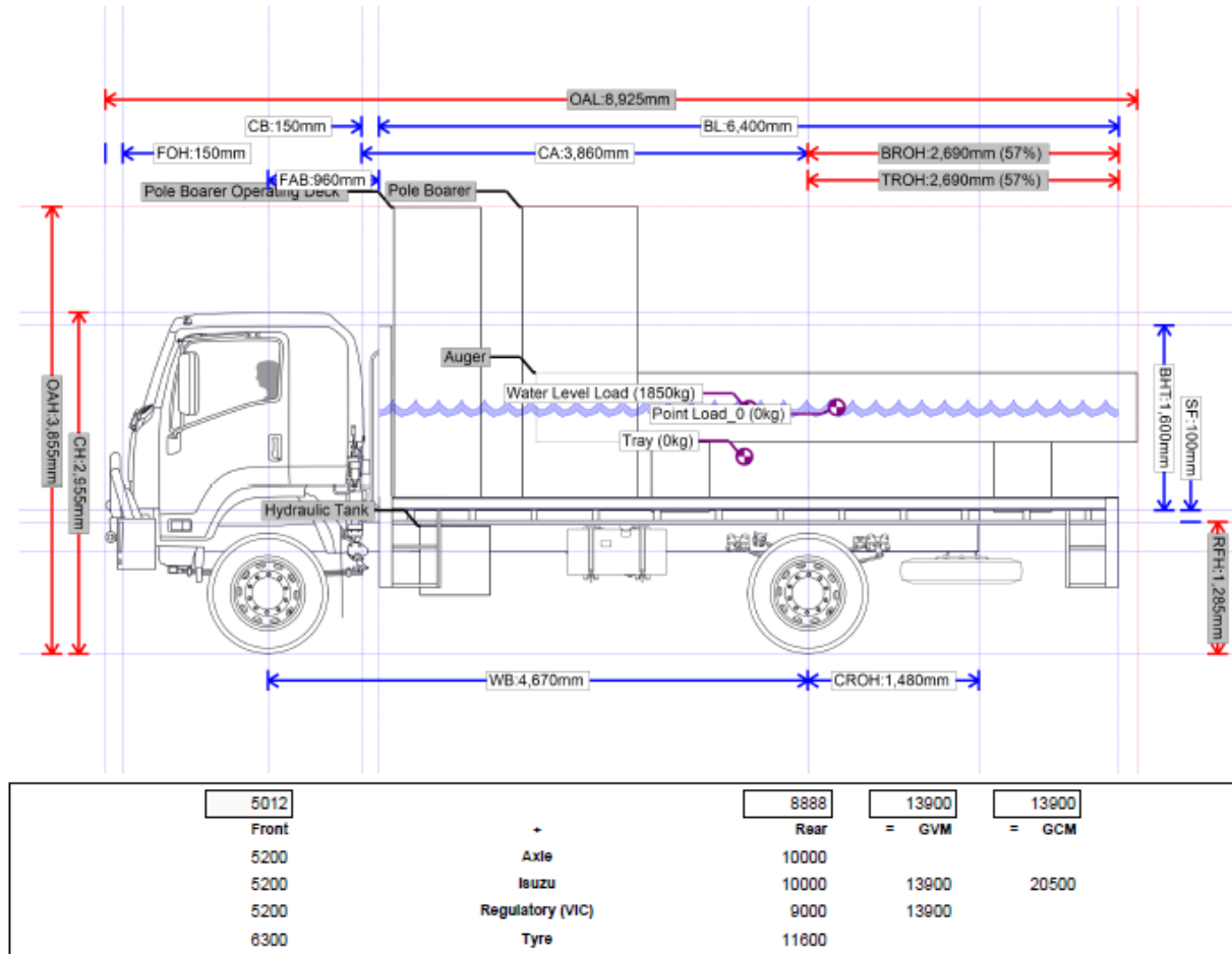
Weight Distribution: 2018 F Series FTS 139-260 4x4 AUTO
